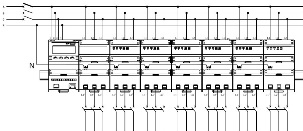
2 channels of three items direct access diagram
